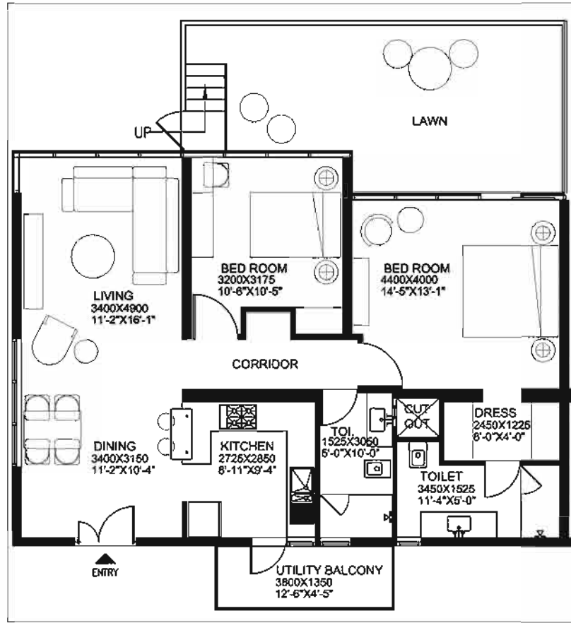
FLOOR PLAN
