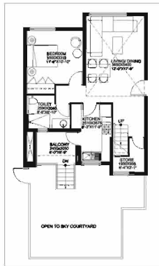
LOWER LEVEL
