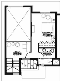
UPPER LEVEL
