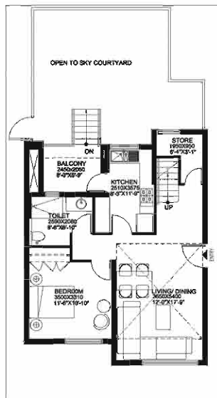
LOWER LEVEL
