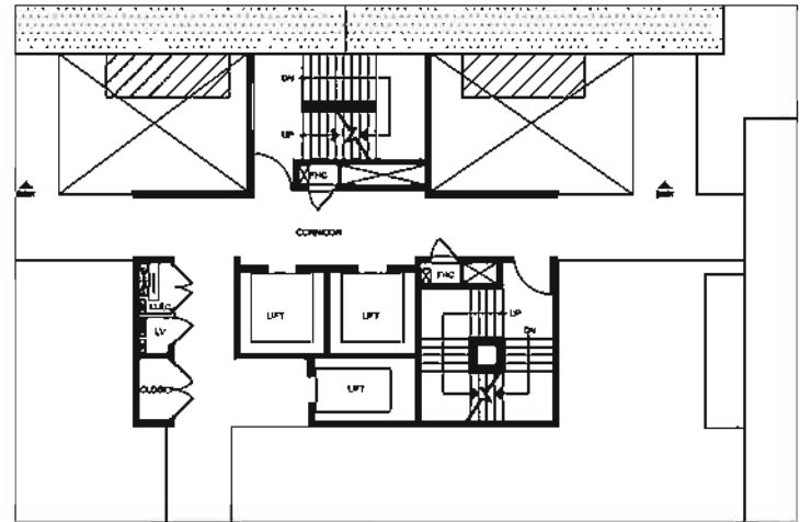
CORE PLAN
