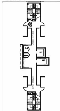
CORE PLAN
