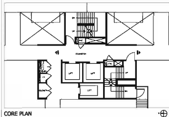
CORE PLAN
