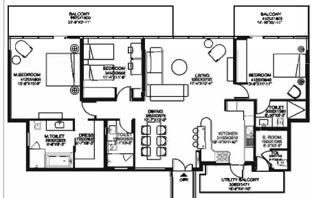
FLOOR PLAN
