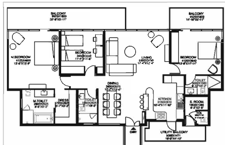
FLOOR PLAN
