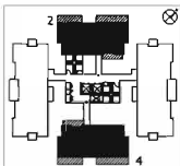
KEY PLAN OF FLOOR 3,6,9,12,15,18,21,24
