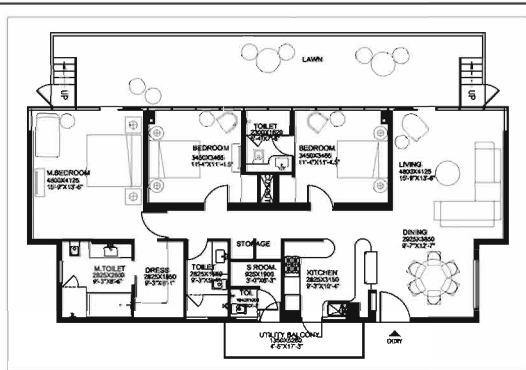
FLOOR PLAN
